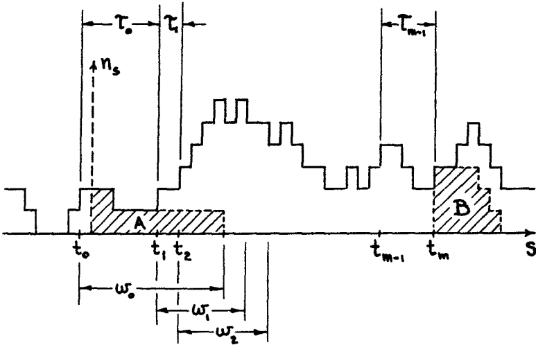
Fig 1. Part of a specific queuing realization \omega , showing the number in the system at time s, n_s , the wait in the system for the r th arrival, w_r , and the interarrival time started by the r th arrival, \tau_r . (The figure is drawn for the case of departure in order of arrival, but this is not required for the proofs in the text)
